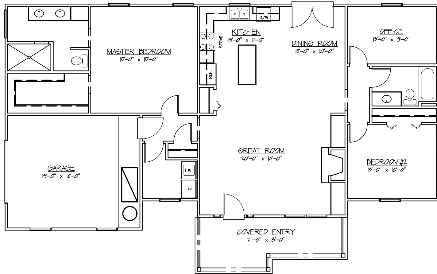
FLOOR PLAN
